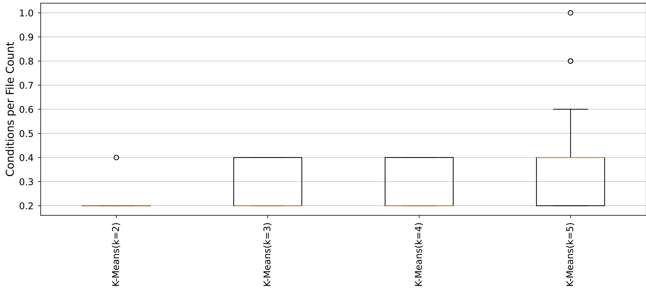
YARA Rules Conditions per File Count Distribution (Cluster45_Size5 dataset)
